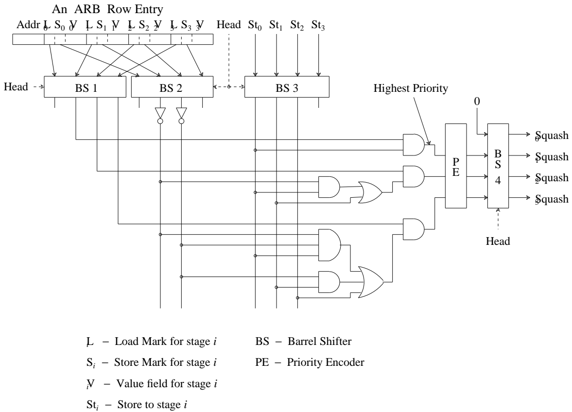
Figure 6.3: Block Diagram of Circuit for Detecting Out-of-sequence Memory Accesses in a 4-stage ARB
