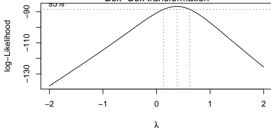
Box-Cox transformation
