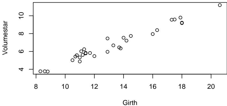
Scatter plot of the transformed data
