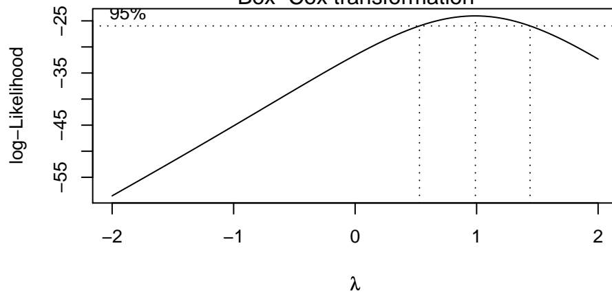
Box-Cox transformation
