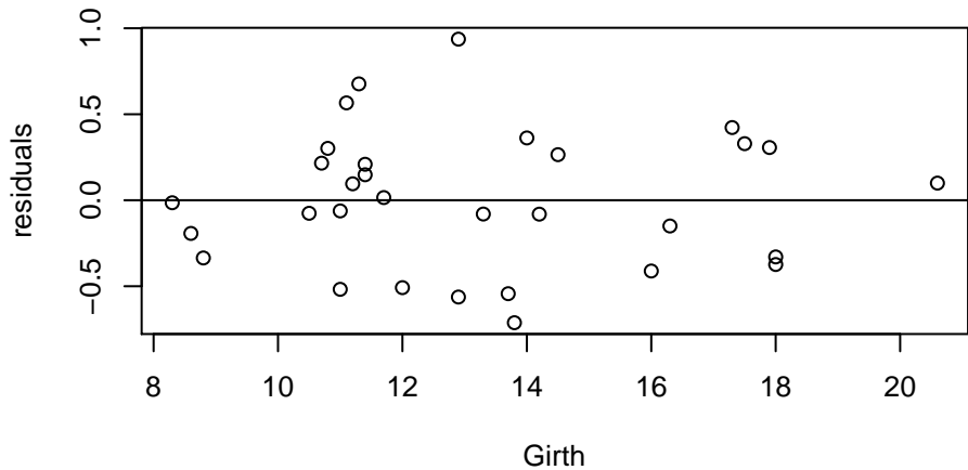
Residual plot from transformed data fit
