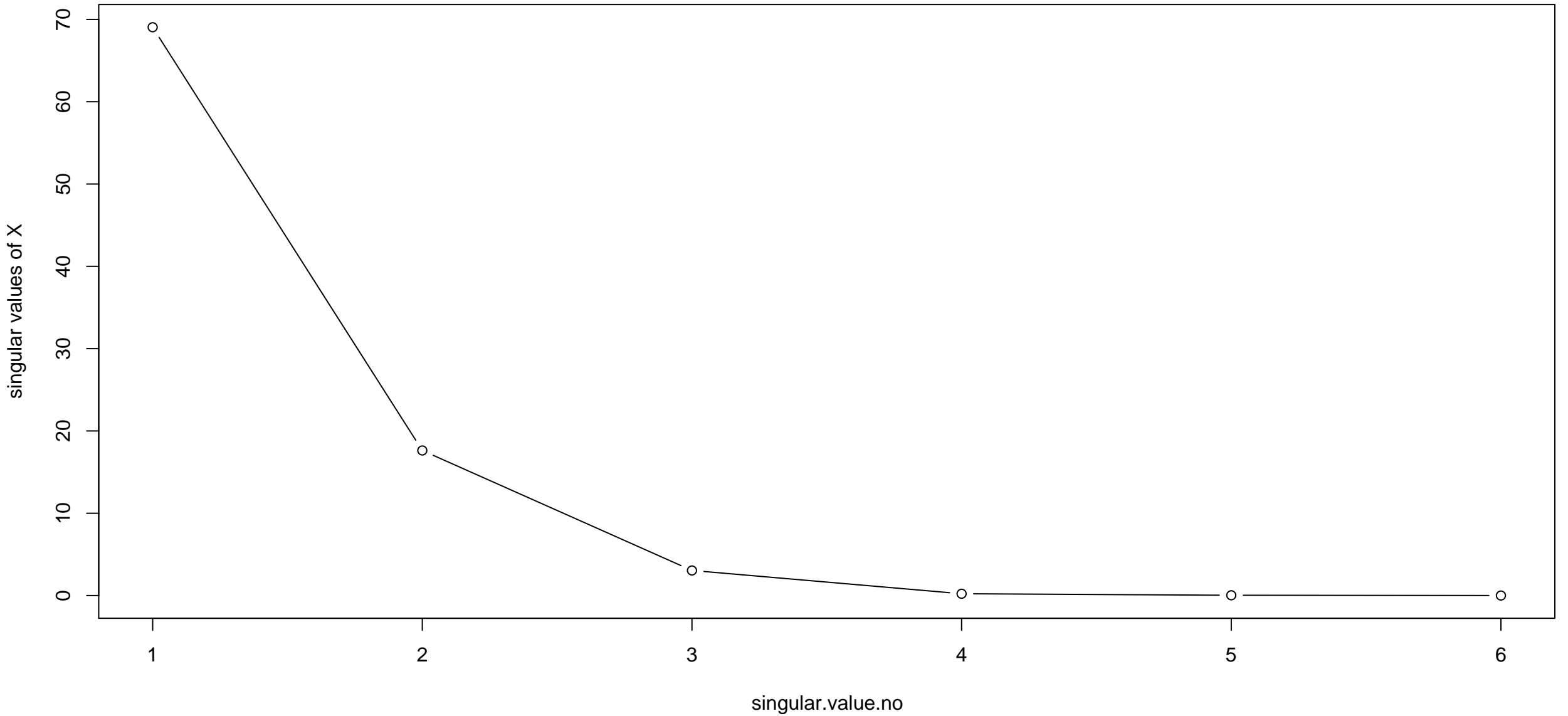
Scree plot to decide on the number of principal components
