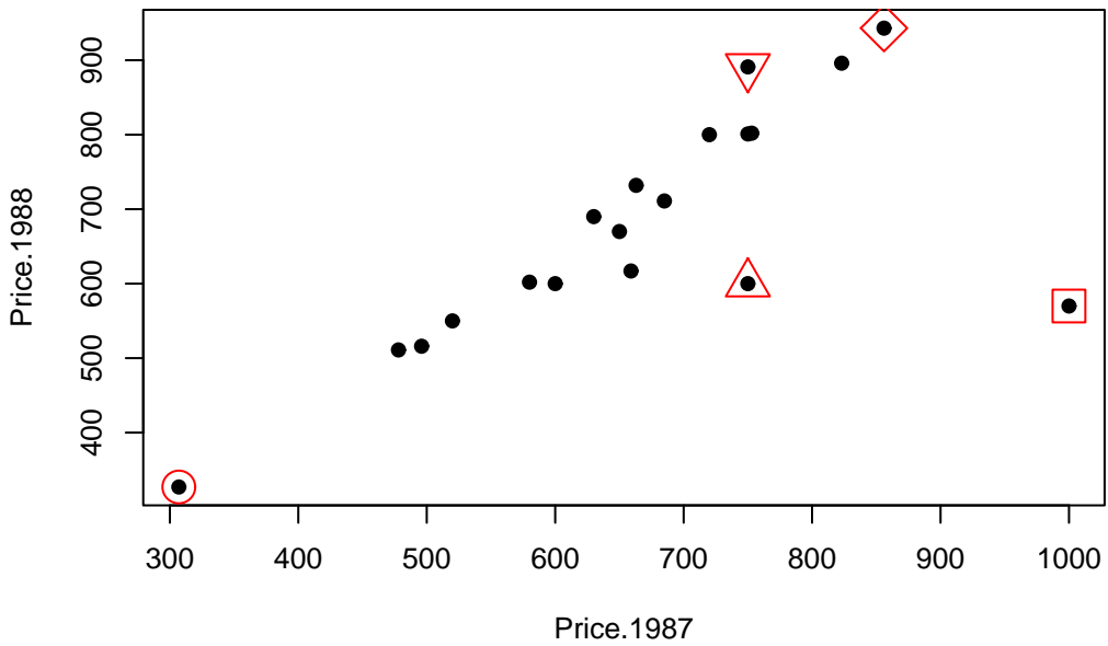
Scatter plot of the data
