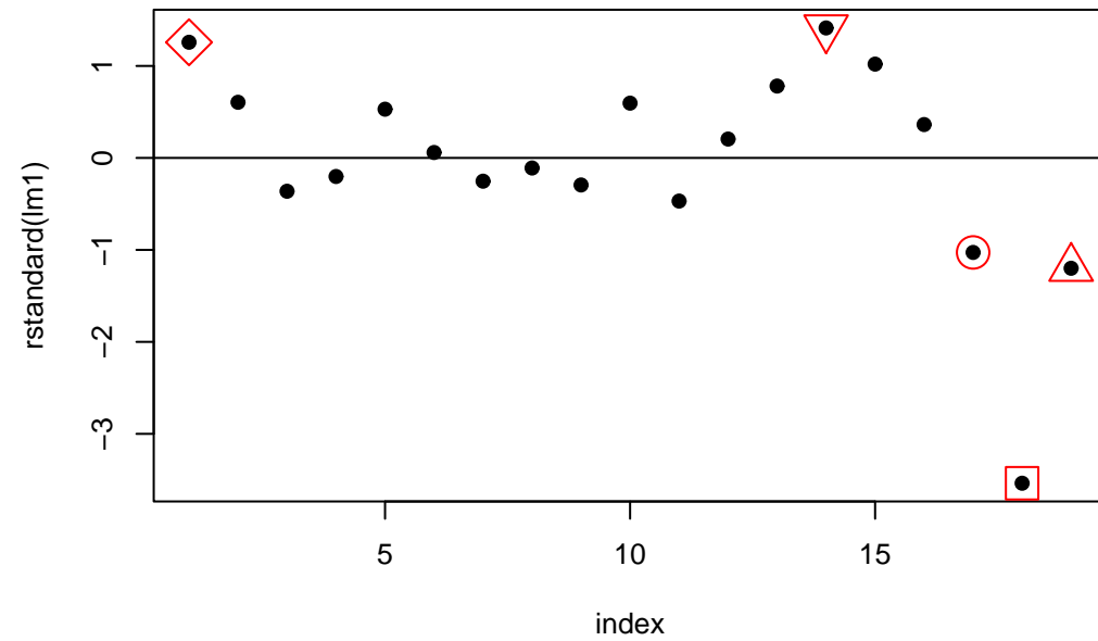
Plot of standardized residuals
