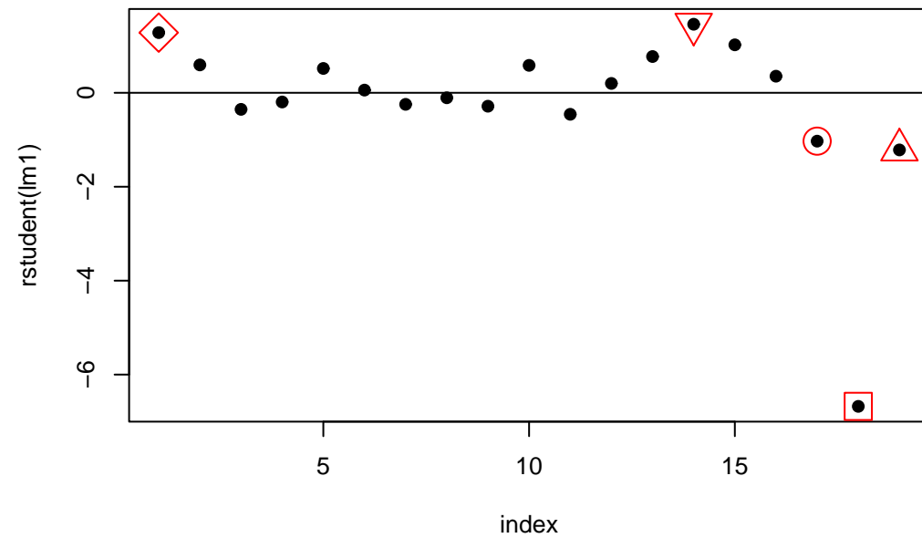
Plot of (externally) studentized residuals
