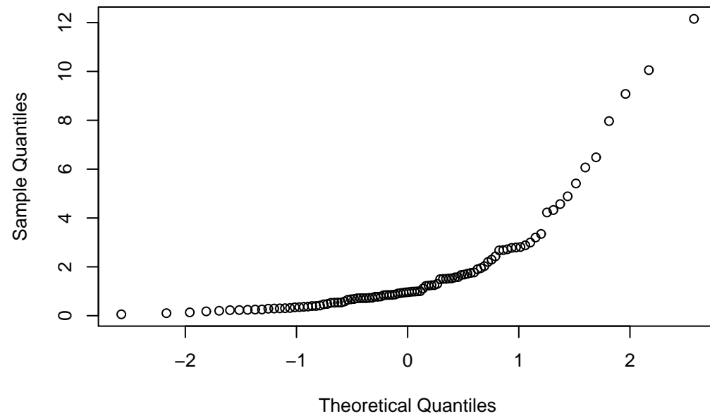
Log-normal: skewed to right
