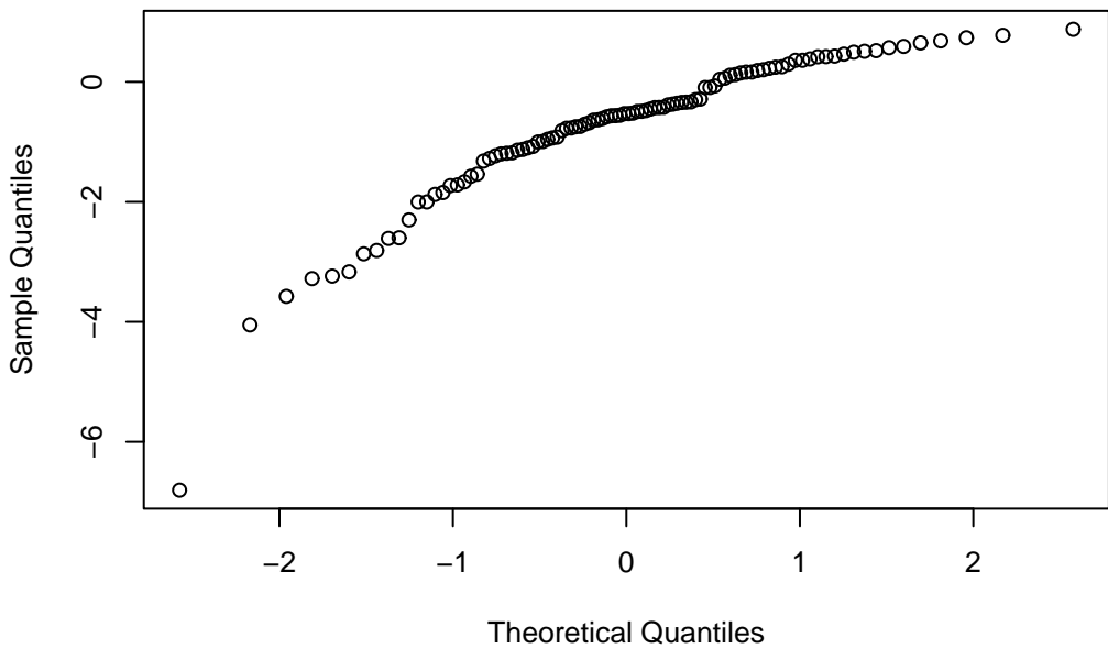
Log-normal: skewed to left
