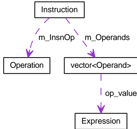
Figure 1: An Instruction and the objects it owns
