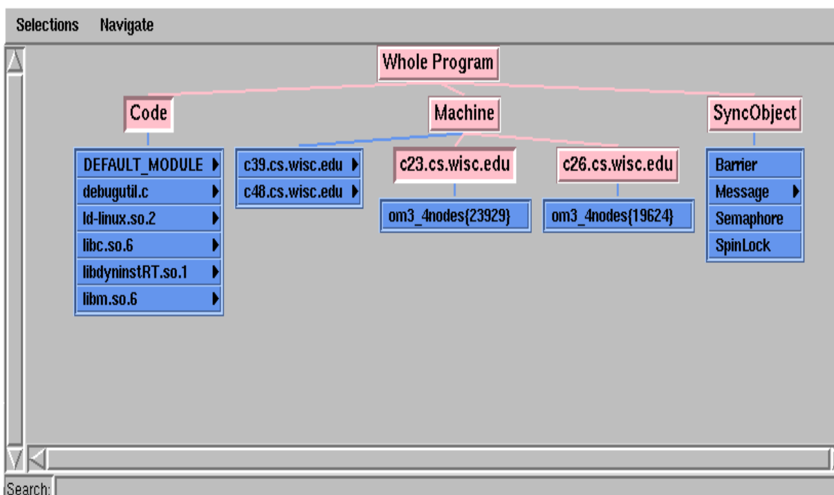
Figure 19: Where Axis after the om3 MPI application process is started
