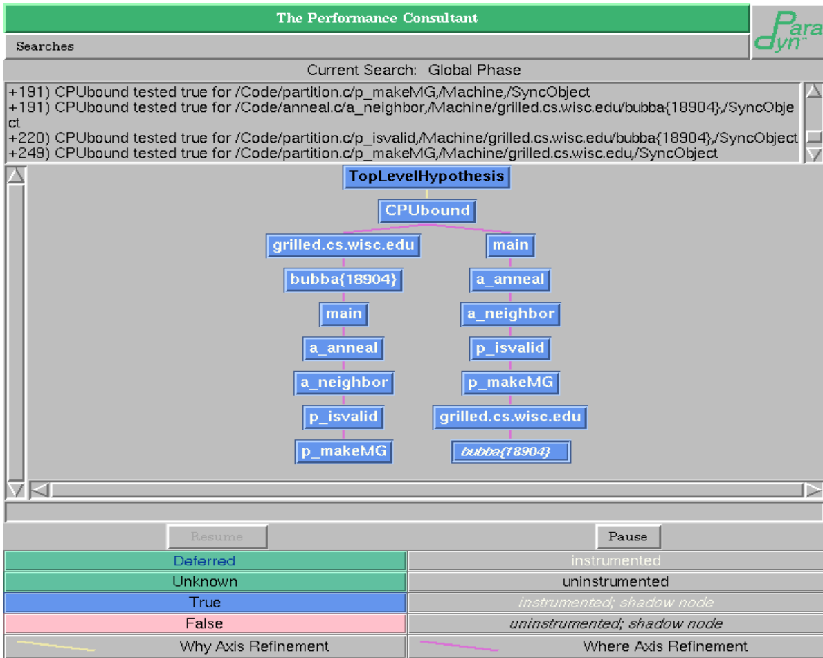
Figure 12: The Search History Graph showing only exigent bubba nodes
