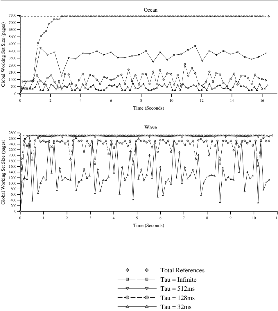
Figure 7. Global working sets for Ocean and Wave.
