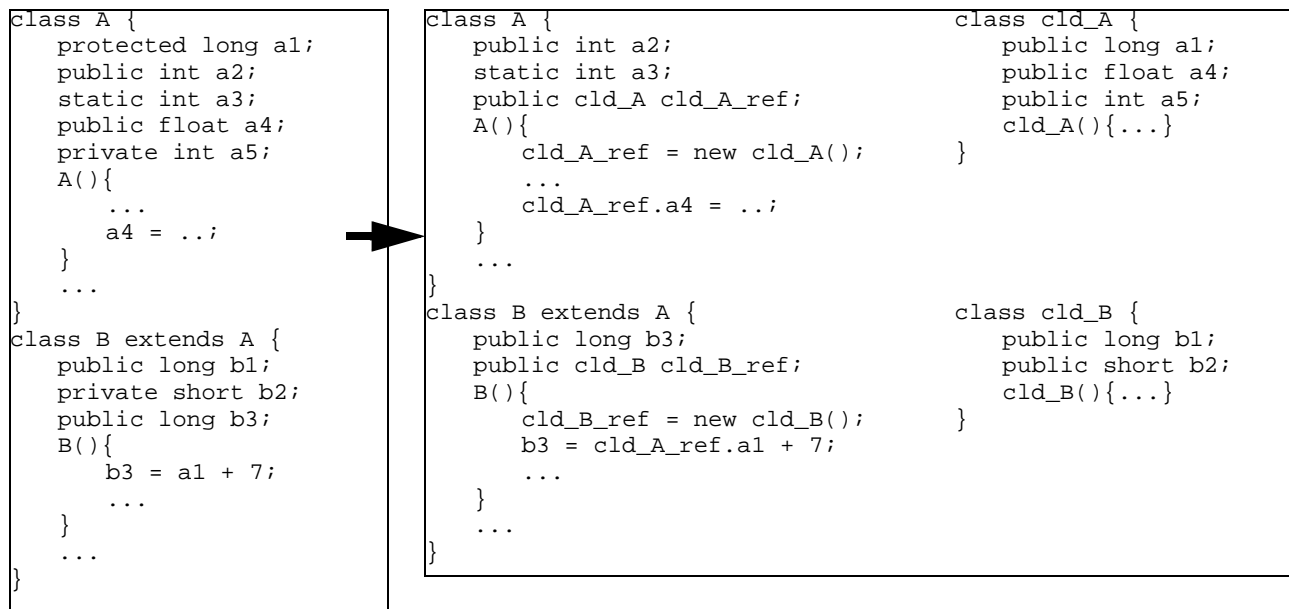
Figure 5. Program transformation.
