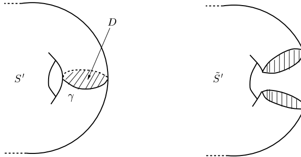
Figure 1: Surgery along a compressing disk
