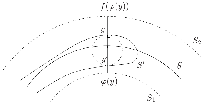
Figure 6: Proof of corollary 5.3.
