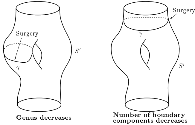
Figure 5: The effects of a surgery on S'
