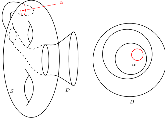
Figure 2: Decreasing the number of components of D \cap \mathcal{S}
