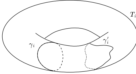
Figure 4: Torus on the boundary of \tilde{M}
