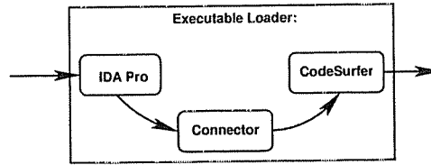
Figure 6: Implementation of executable loader module.
