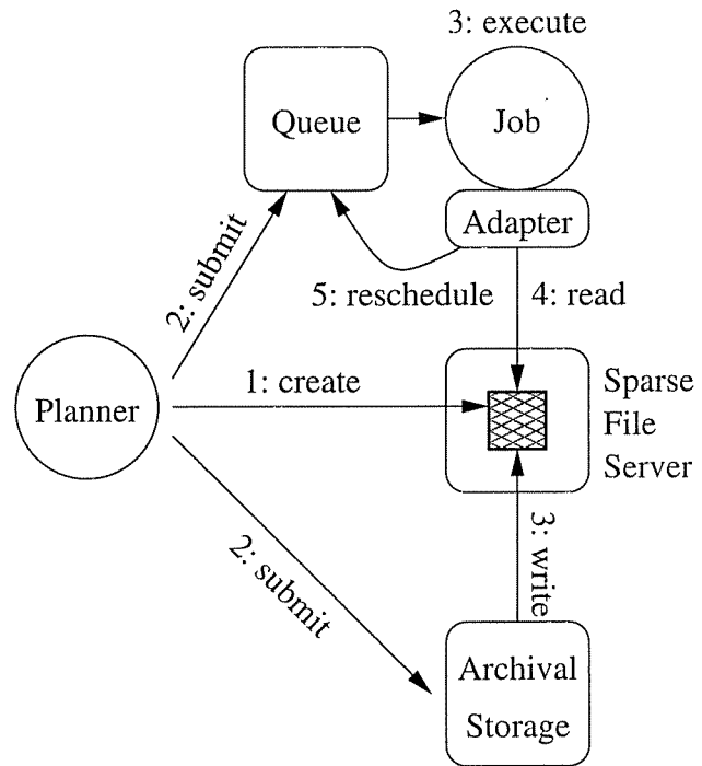
Figure 4. Staged Input
