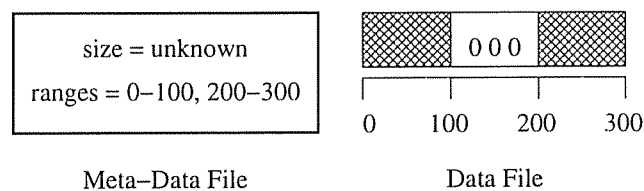
Figure 8. Sparse File Implementation
