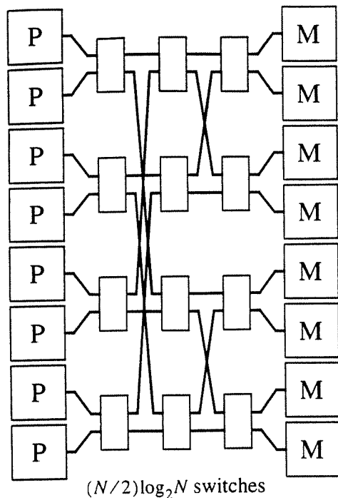
Figure 1. Dancehall architectures
