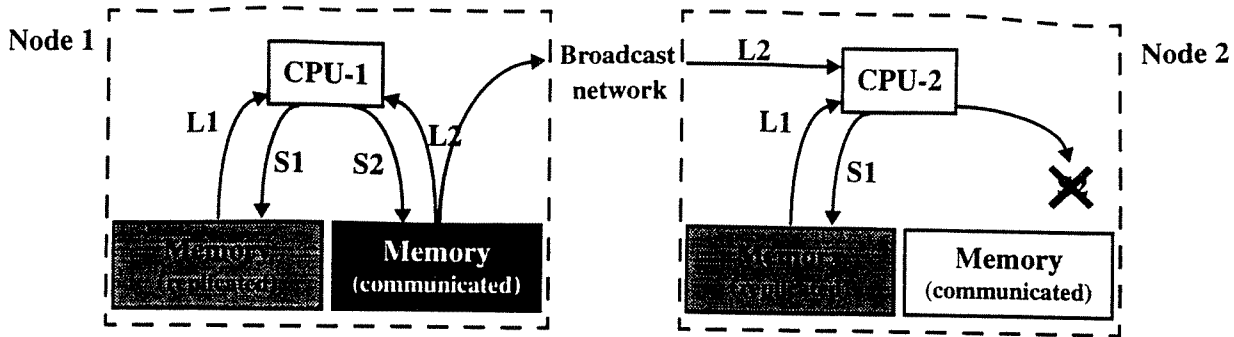
Figure 4. Replicated versus communicated main memory
