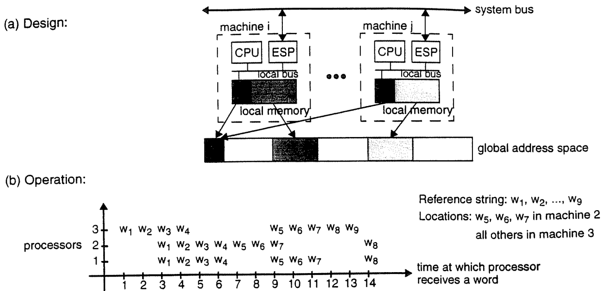
Figure 5. Design and operation of the ESP Massive Memory Machine (taken from [8])
