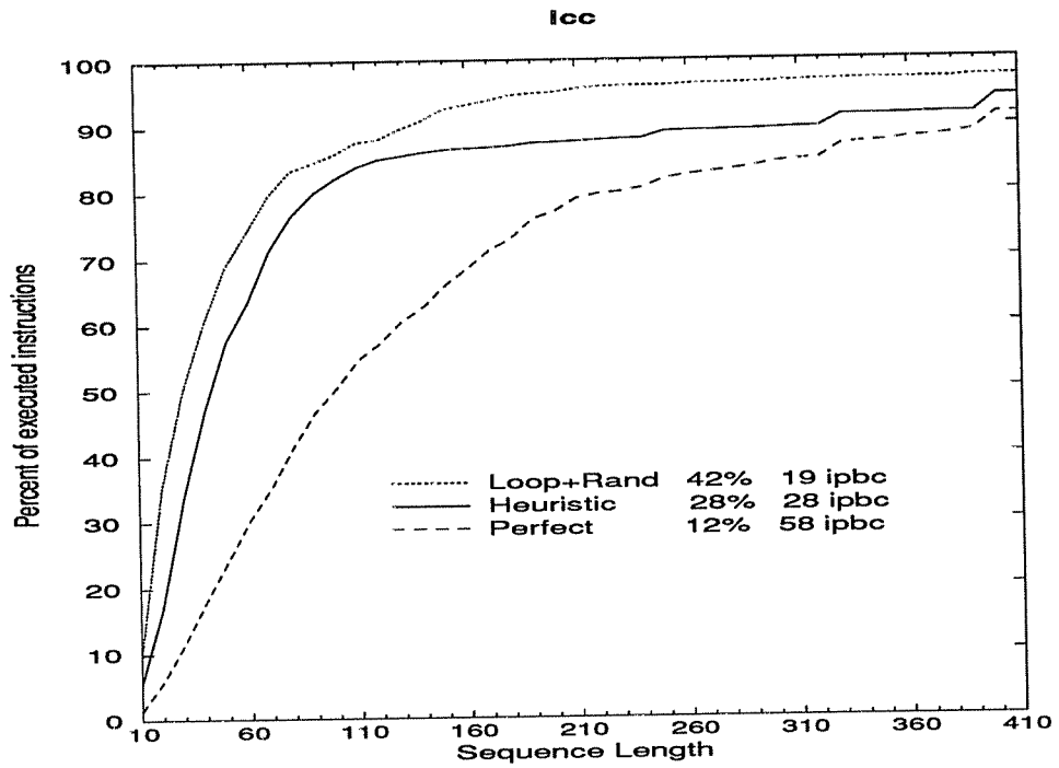
Graph 8. lcc : cumulative distribution of sequence lengths.
