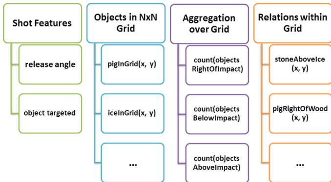
Figure 2: Features represented in AngryBirdsGridExamples . “Counting an object” counts the number of cells containing that object. Relations like stoneAboveIce(x, y) are true if cell x - y contains ice and some cell at or above y in column x contains a stone.
