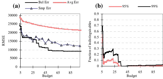
Figure 7. Basic bellwether analysis of the mail order dataset
