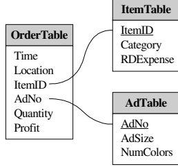
Figure 1. Data schema of the motivating example
