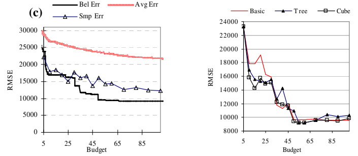
Figure 8. Bellwether-based prediction on the mail order dataset
