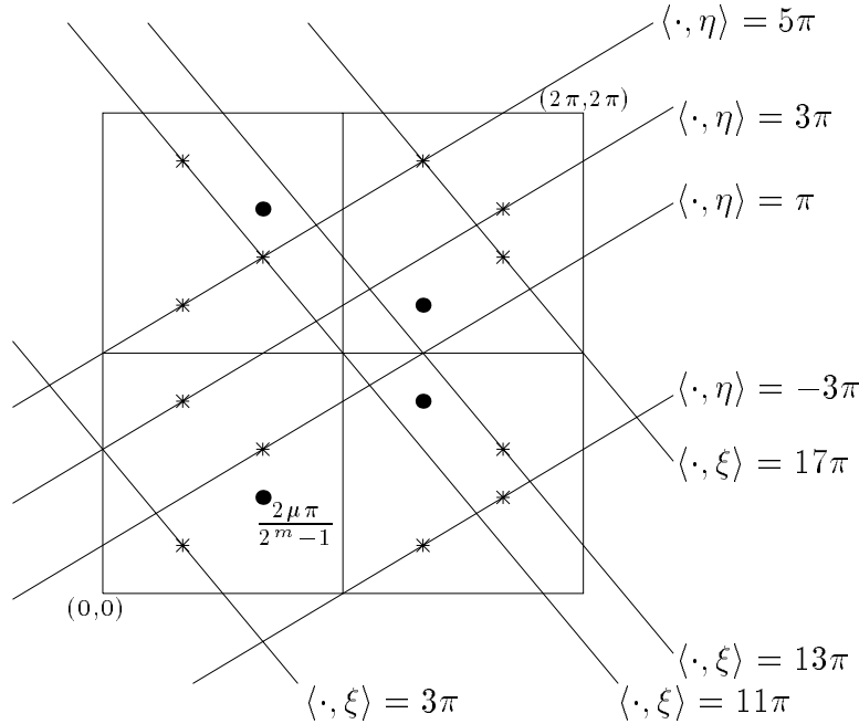
Figure 1. Contaminating zero set with \frac{2\mu\pi}{2^m - 1} = \left(\frac{2\pi}{3}, \frac{2\pi}{5}\right) from Example 4.3.
